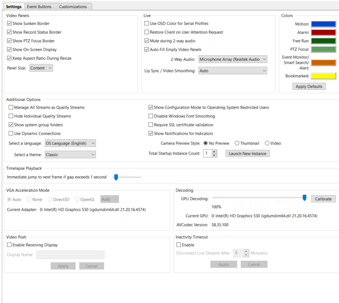
Figure 22: Client configuration
